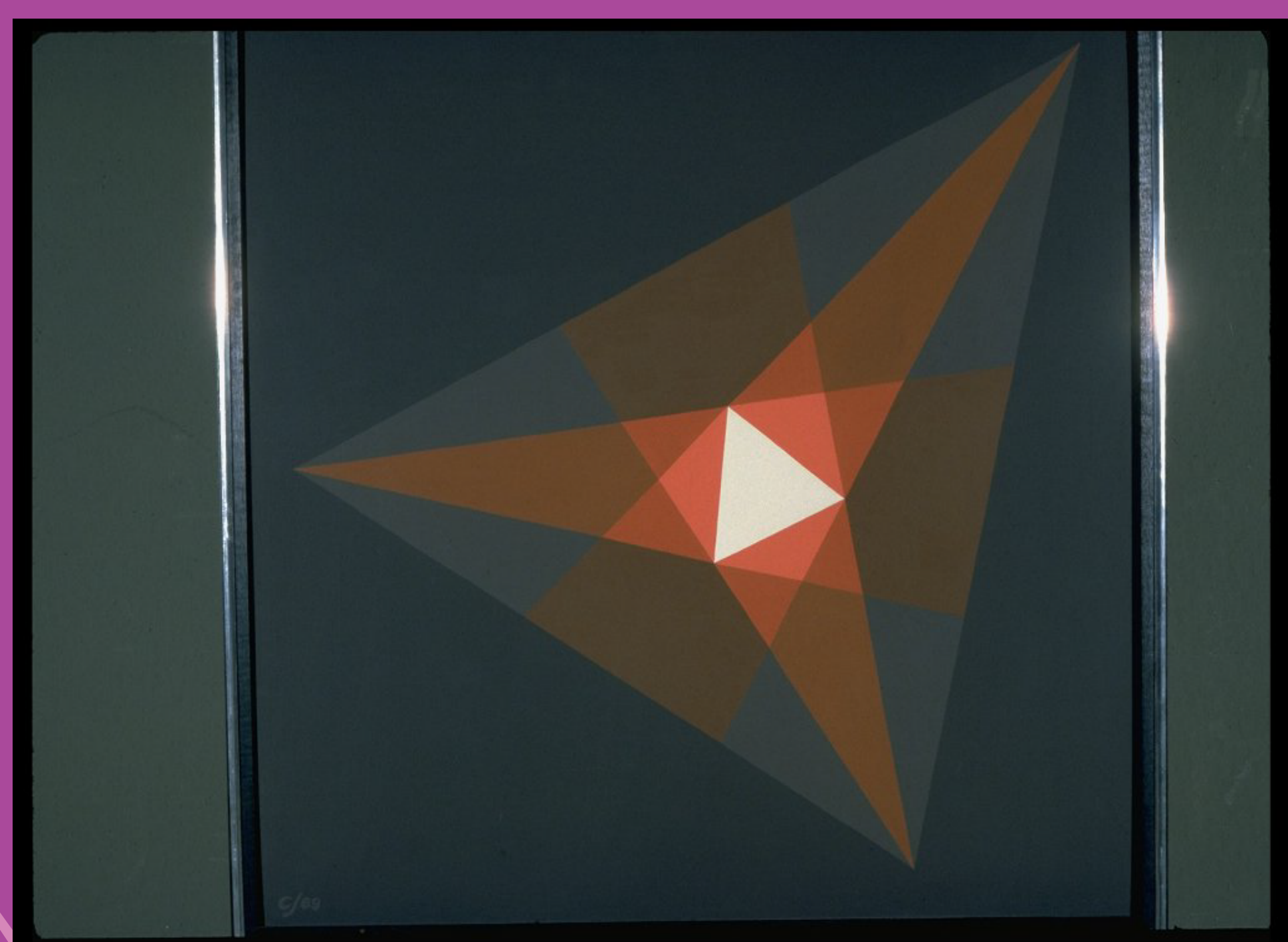
Squared Circles
