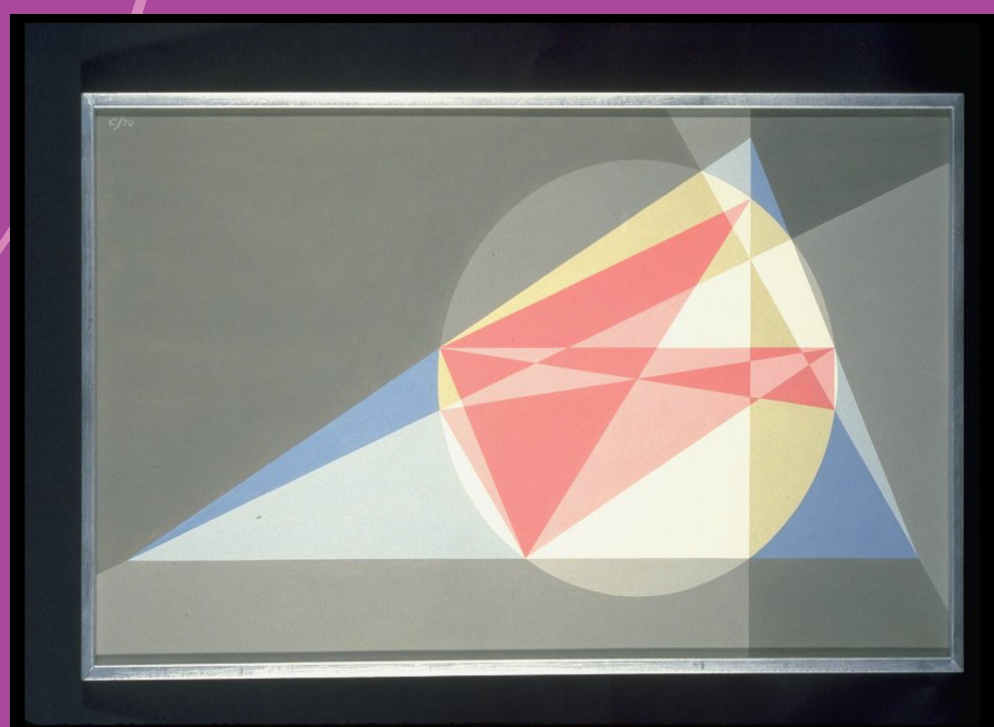
Morley's Triangles
